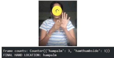
Figure 11: Hand Location Detection Using Hand Landmarks with predicted HamNoSys label hampalm .
