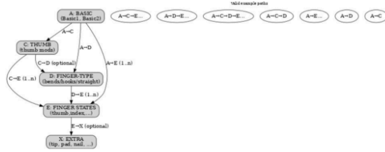
Figure 2 : Hierarchical Structure of HamNoSys Handshape Components
